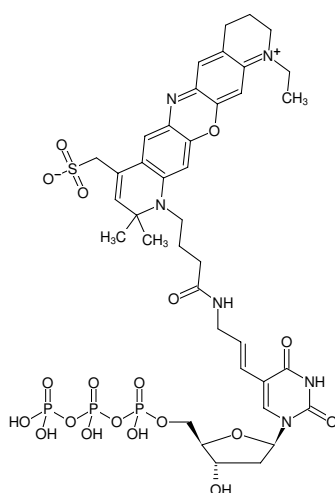
Structural formula of Atto680 NT Labeling Kit
