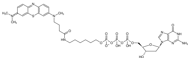
Structural formula of \gamma -(6-Aminoethyl)-dGTP-ATTO-MB2
