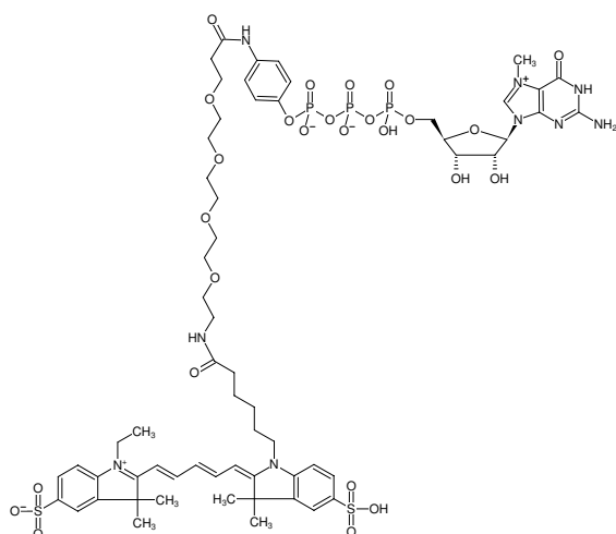
Structural formula of m 7 GTP-γ-aminophenyl-PEG 4 - Cy5
