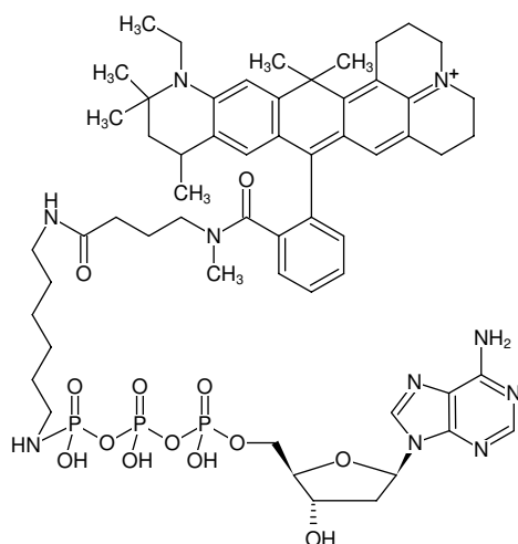
Structural formula of \gamma -[(6-Aminoethyl)-imido]-dATP-ATTO-647N
