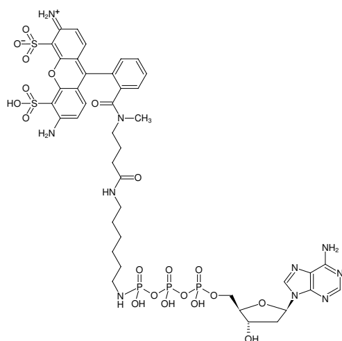
Structural formula of \gamma -[(6-Aminohexyl)-imido]-dATP-ATTO-488
