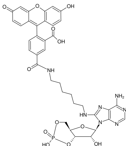
Structural formula of 8-(6-Aminoethyl)-amino-cAMP-5-FAM
