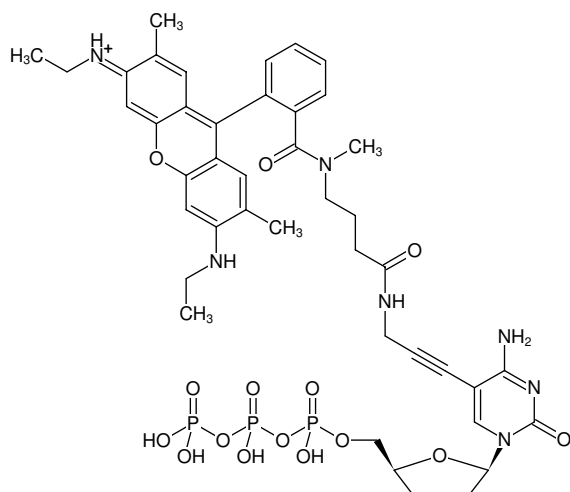
Structural formula of 5-Propargylamino-ddCTP-ATTO-Rho6G
