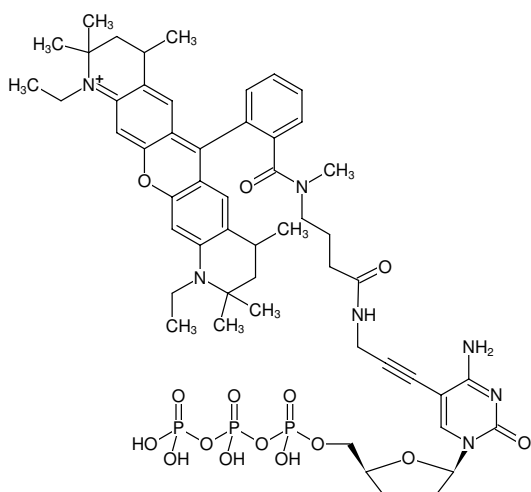
Structural formula of 5-Propargylamino-ddCTP-ATTO-Rho12
