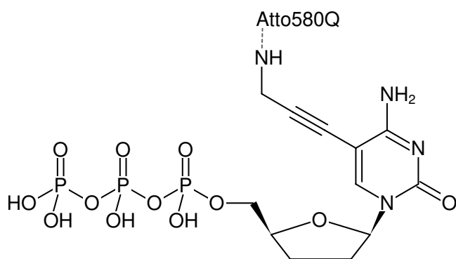
Structural formula of 5-Propargylamino-ddCTP-ATTO-580Q
