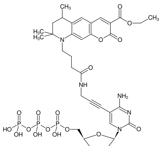
Structural formula of 5-Propargylamino-ddCTP-ATTO-425
