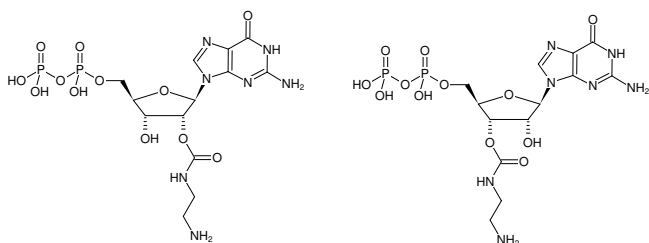
Structural formula of EDA-GDP
