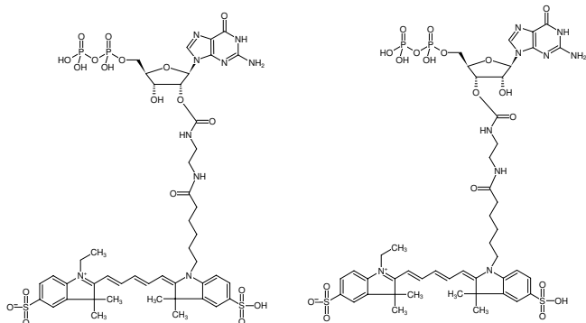
Structural formula of EDA-GDP-Cy5
