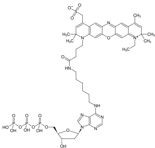
Structural formula of N 6 -(6-Aminohexyl)-dATP-ATTO-700
