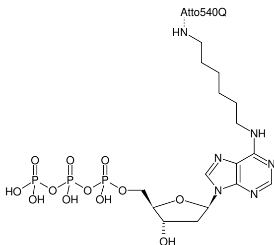
Structural formula of N 6 -(6-Aminoheptyl)-dATP-ATTO-540Q
