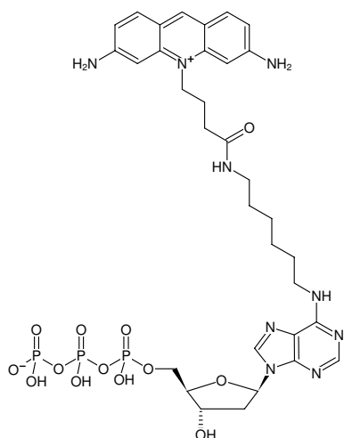
Structural formula of N 6 -(6-Aminoheptyl)-dATP-ATTO-465
