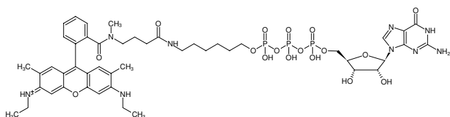
Structural formula of \gamma -(6-Aminoethyl)-GTP-ATTO-Rho6G
