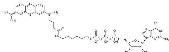
Structural formula of \gamma -(6-Aminoethyl)-GTP-ATTO-MB2
