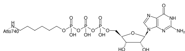
Structural formula of \gamma -(6-Aminoethyl)-GTP-ATTO-740
