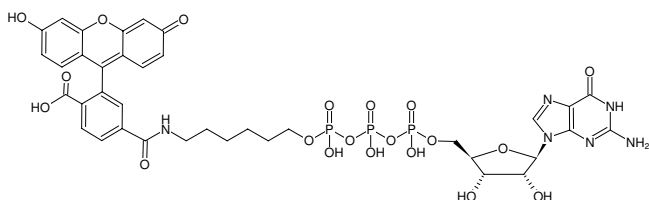
Structural formula of \gamma -(6-Aminoethyl)-GTP-6-FAM
