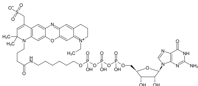
Structural formula of \gamma -(6-Aminoethyl)-GTP-ATTO-680
