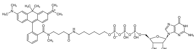
Structural formula of \gamma -(6-Aminoethyl)-GTP-ATTO-620
