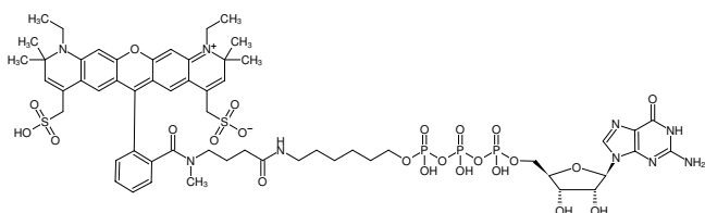
Structural formula of \gamma -(6-Aminoethyl)-GTP-ATTO-594
