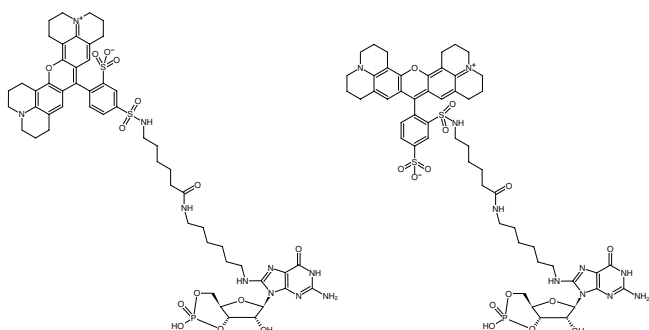
Structural formula of 8-(6-Aminoethyl)-amino-cGMP-Texas Red
