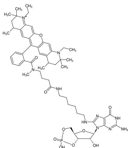
Structural formula of 8-(6-Aminoethyl)-amino-cGMP-ATTO-Rho12
