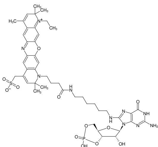
Structural formula of 8-(6-Aminoethyl)-amino-cGMP-ATTO-700
