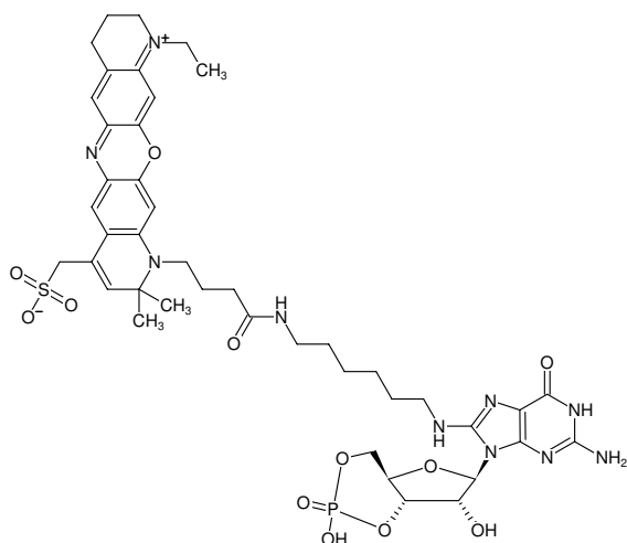
Structural formula of 8-(6-Aminoethyl)-amino-cGMP-ATTO-680
