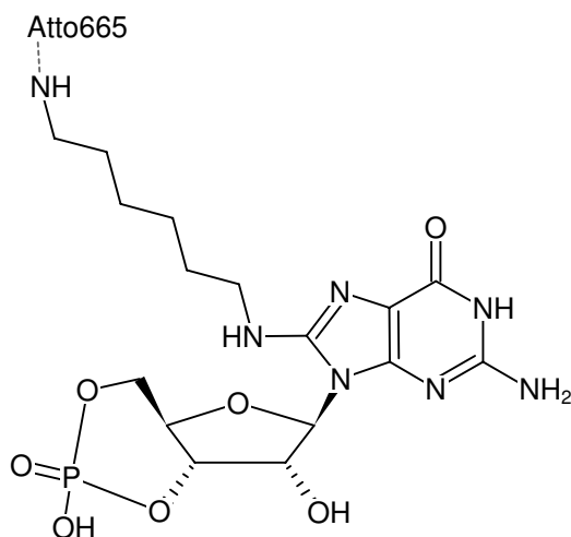
Structural formula of 8-(6-Aminoethyl)-amino-cGMP-ATTO-665
