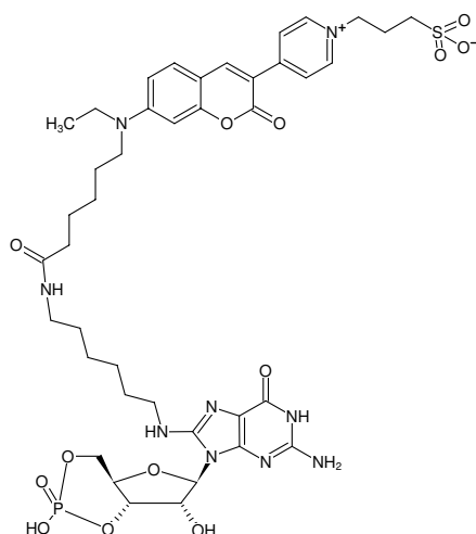
Structural formula of 8-(6-Aminoheptyl)-amino-cGMP-DY-485XL
