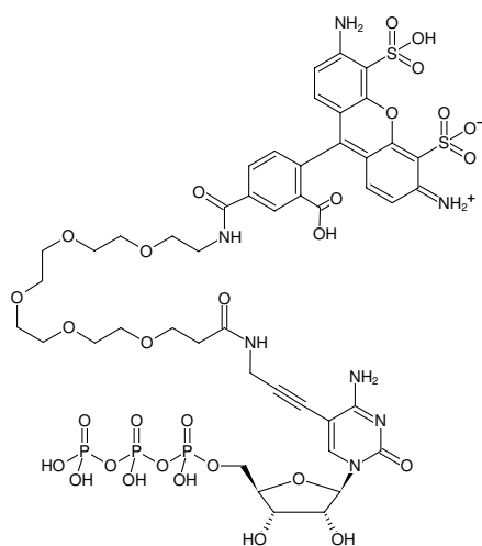
Structural formula of 5-Propargylamino-CTP-PEG 5 -AF488
