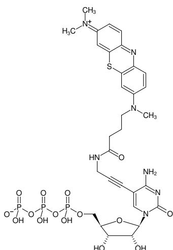
Structural formula of 5-Propargylamino-CTP-ATTO-MB2
