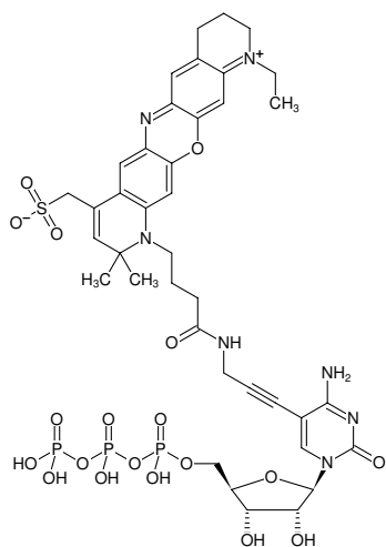
Structural formula of 5-Propargylamino-CTP-ATTO-680
