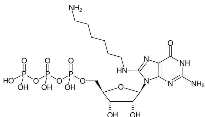
Structural formula of 8-(6-Aminoethyl)-amino-GTP
