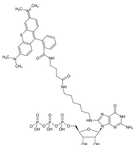
Structural formula of 8-(6-Aminoheptyl)-amino-GTP-ATTO-Thio12
