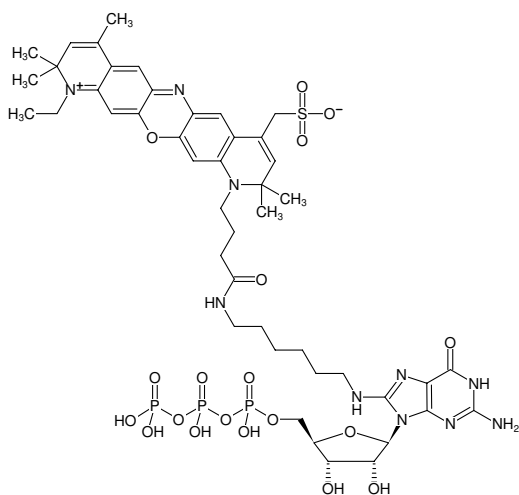
Structural formula of 8-(6-Aminoethyl)-amino-GTP-ATTO-700
