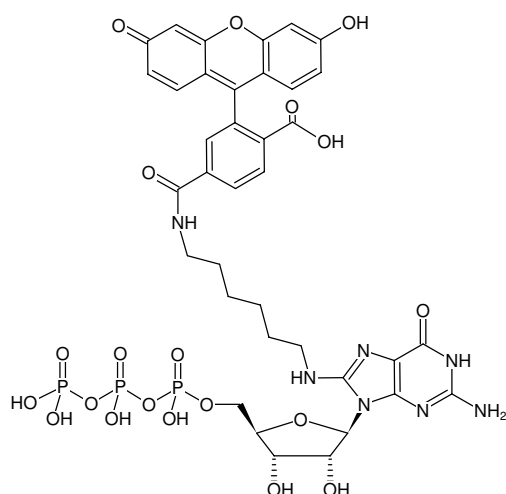
Structural formula of 8-(6-Aminoethyl)-amino-GTP-6-FAM
