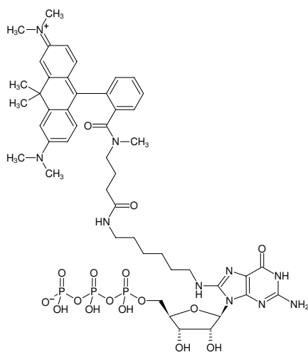
Structural formula of 8-(6-Aminoethyl)-amino-GTP-ATTO-620
