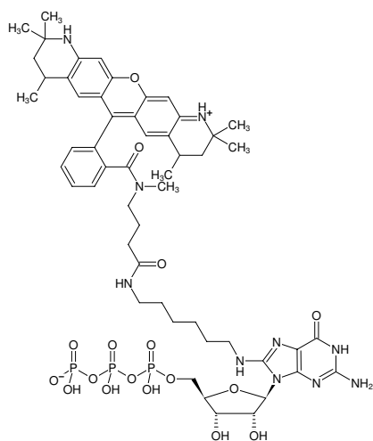
Structural formula of 8-(6-Aminoethyl)-amino-GTP-ATTO-550
