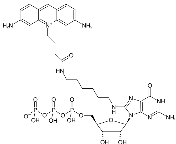
Structural formula of 8-(6-Aminoethyl)-amino-GTP-ATTO-465
