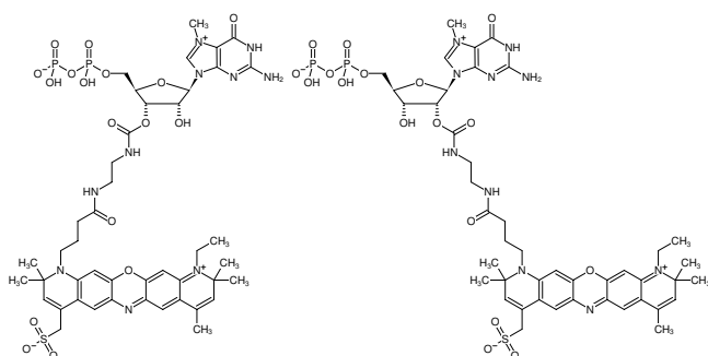
Structural formula of EDA-m 7 GDP-ATTO-700
