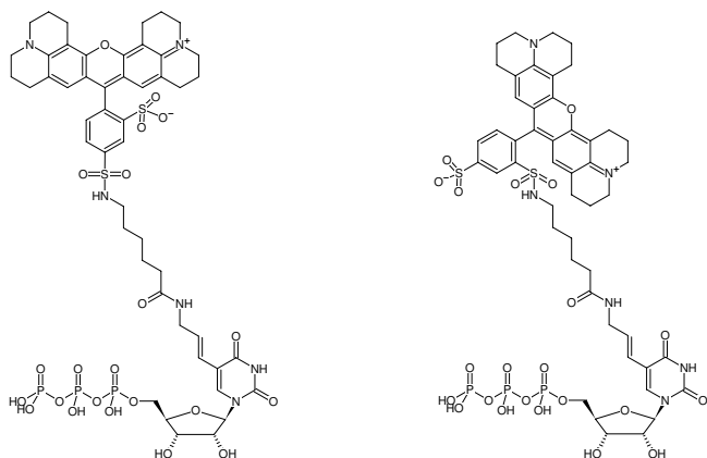
Structural formula of Aminoallyl-UTP-Texas Red
