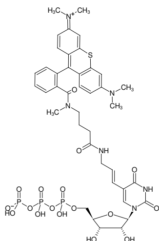
Structural formula of Aminoallyl-UTP-ATTO-Thio12
