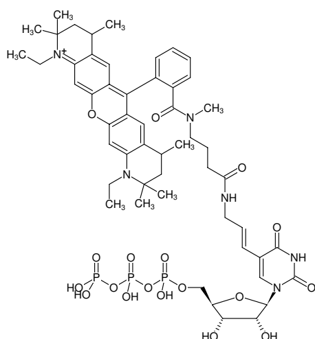
Structural formula of Aminoallyl-UTP-ATTO-Rho12
