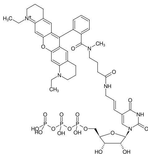
Structural formula of Aminoallyl-UTP-ATTO-Rho11
