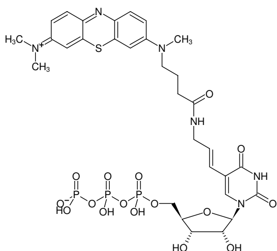
Structural formula of Aminoallyl-UTP-ATTO-MB2
