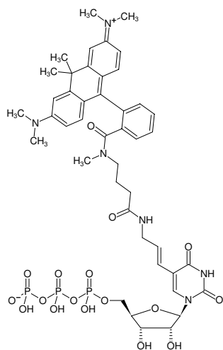
Structural formula of Aminoallyl-UTP-ATTO-620
