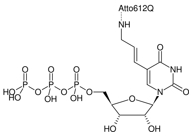
Structural formula of Aminoallyl-UTP-ATTO-612Q
