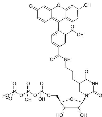
Structural formula of Aminoallyl-UTP-5-FAM
