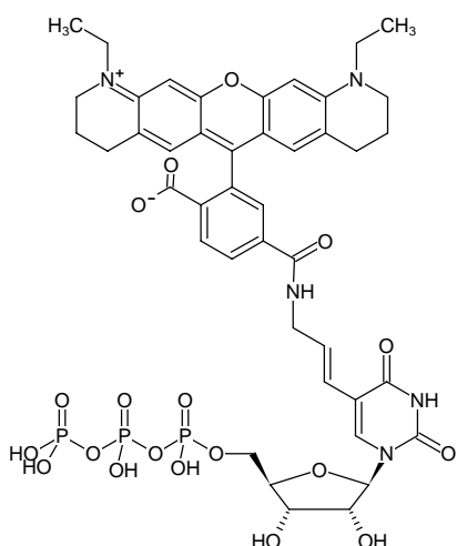
Structural formula of Aminoallyl-UTP-ATTO-565
