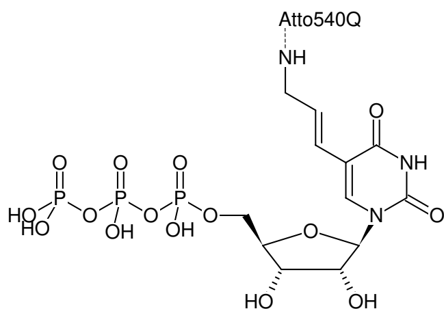
Structural formula of Aminoallyl-UTP-ATTO-540Q
