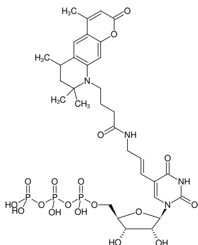
Structural formula of Aminoallyl-UTP-ATTO-390
